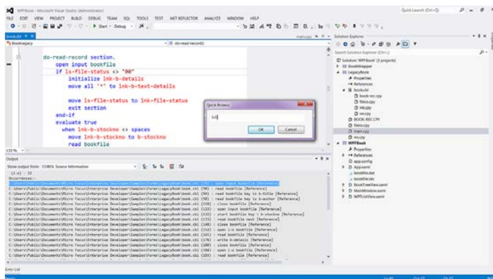
COBOL Source Information output from Visual Studio showing all instances of file IO usage within a program
